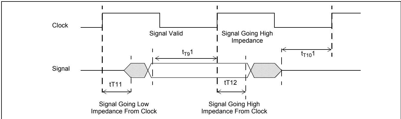
Figure 20 - Tri-State Timing
